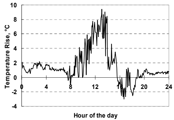
Fig. 7. Increase in air temperature above the ambient at a location 0.3 m above PV panel (28/05/2002).
