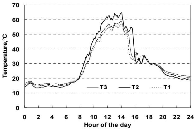
Fig. 5. Temperatures measured on the back surfaces of the PV panels (28/05/2002).
