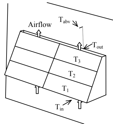
Fig. 4. Location of measurement points, ( T_1 , T_2 , and T_3 measured on the backside of the PV panels).
