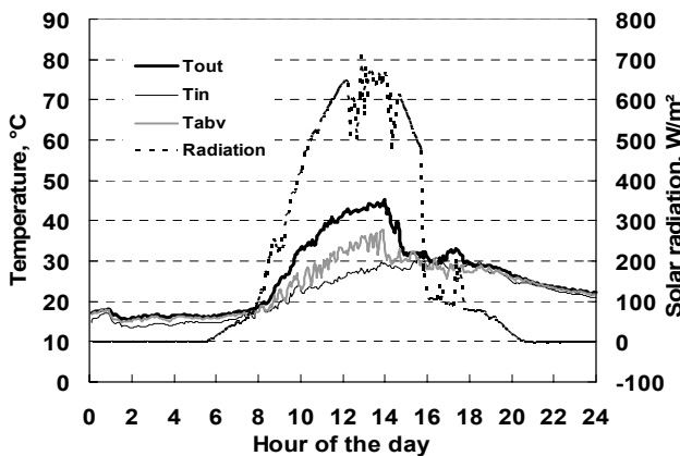
Fig. 6. Air temperature adjacent to the PV array and solar radiation levels on 28/05/2002.
