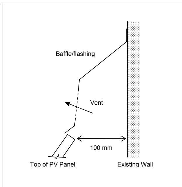
Fig. 13. Configuration of the baffle/flashing used above the PV arrays, (side view, not to scale).
