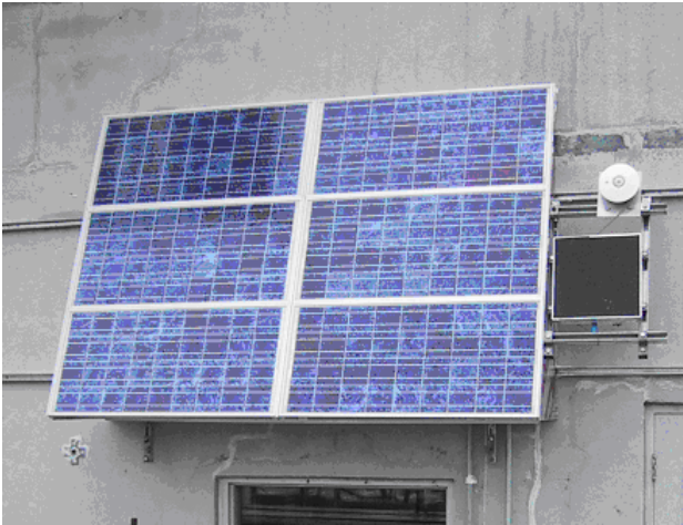
Fig 2. Front view of the “mockup” test section of the proposed BIPV configuration.
