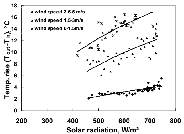
Fig. 8. Air temperature rise, ( T_{out} - T_{in} ), as a function of solar radiation and wind speed.
