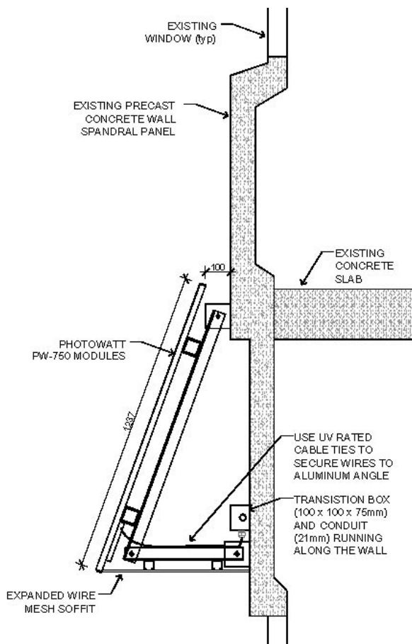
Fig. 10. Revised specification for the attachment of the PV modules to the building wall (Halsall, 2002).
