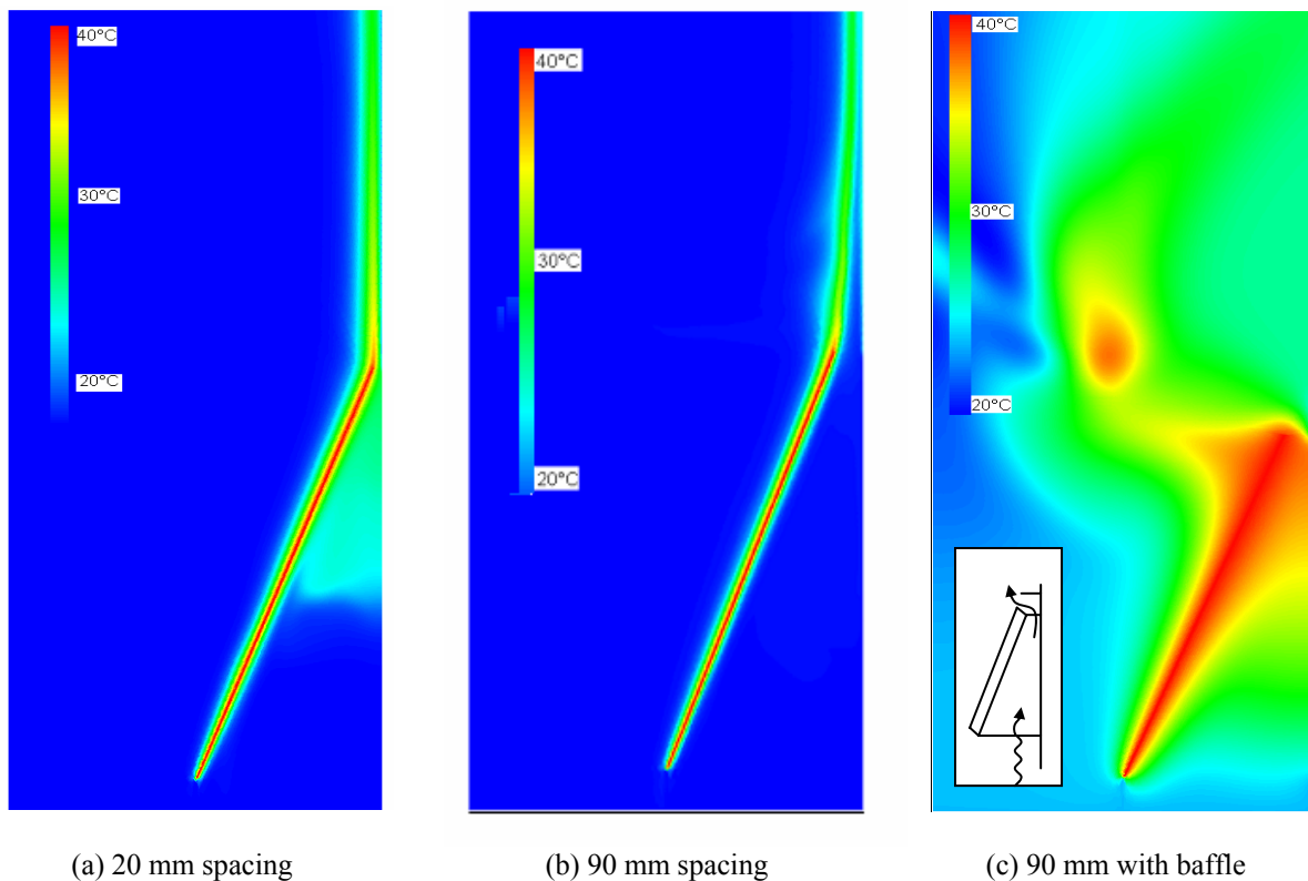
Fig. 9. Relative temperatures and flow field around the PV array for an assumed PV panel temperature of 40°C, an ambient temperature of 20°C, and a 24°C wall temperature above the array. Results are shown for cases: (a) panel to wall distance = 20 mm; (b) panel to wall distance = 90 mm and; (c) 90 mm gap with deflector baffle located 90 mm above the array.
